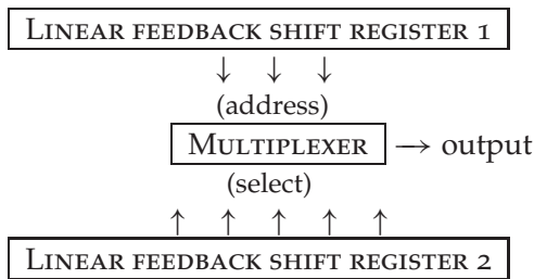
Figure 22.4: The multiplexer generator
