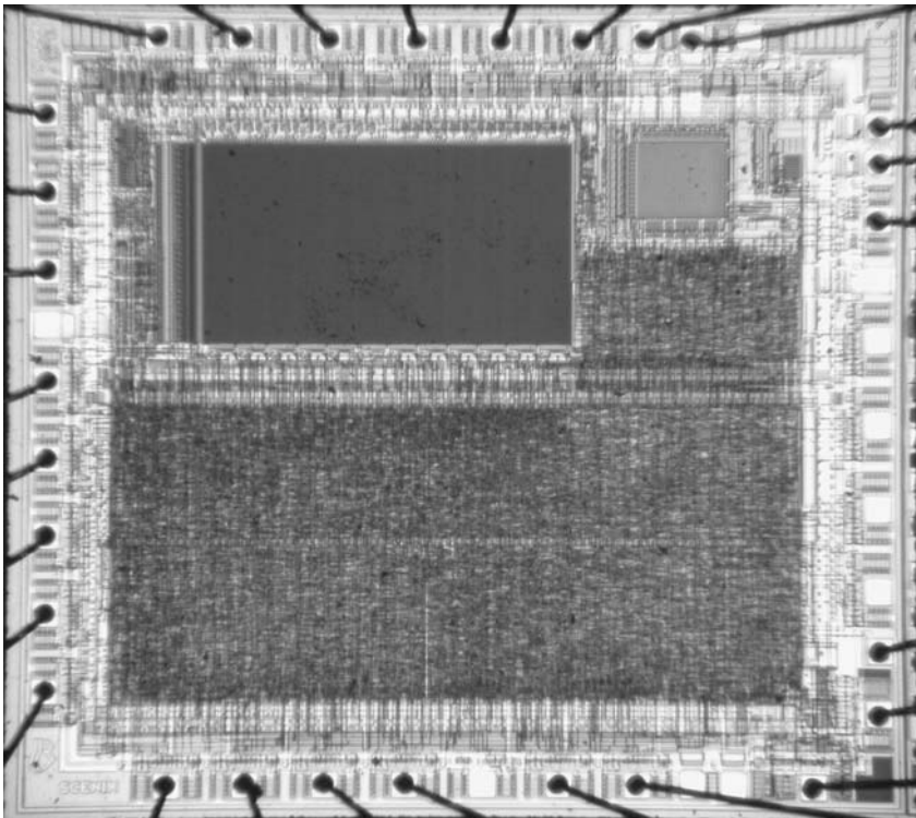
Figure 16.8: SX28 microcontroller with 'glue logic' (courtesy of Sergei Skorobogotov)
