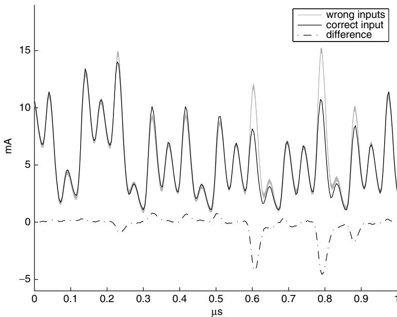
Figure 17.1: Plot of the current measured during 256 single attempts to guess the first byte of a service password stored in the microcontroller at the heart of a car immobilizer (courtesy of Markus Kuhn and Sergei Skorobogatov).
