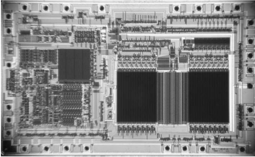
Figure 16.7: MC68HC705P6A microcontroller (courtesy of Sergei Skorobogotov)
