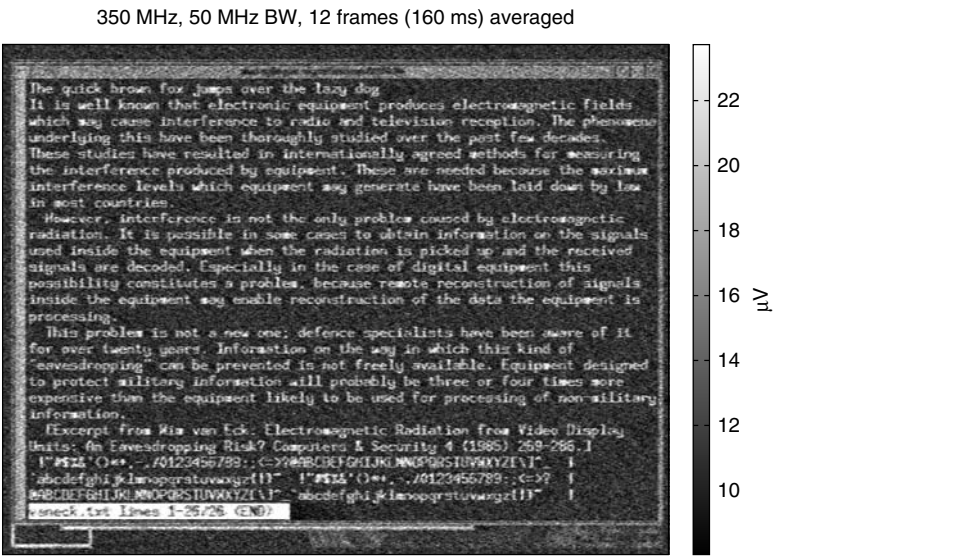
Figure 17.2: RF signal from a Toshiba laptop reconstructed several rooms away, through three plasterboard walls (courtesy of Markus Kuhn [752]).
